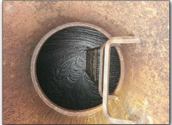
2- Entrained air / froth seen immediately following bunkering - ullage 171 cm
